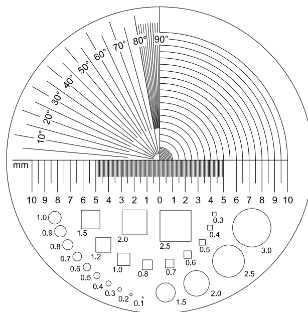
7527-D2底板刻线 (0-5mm分度值0.1mm, 5-10mm分度值0.5mm)
